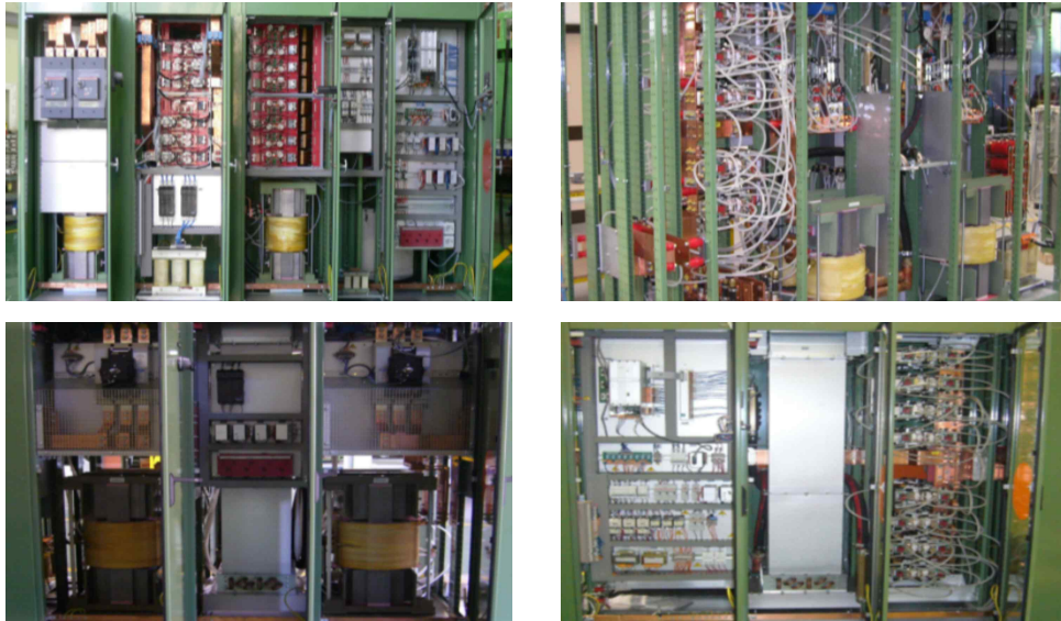
Inside of Converter
