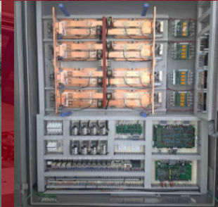
IGBT Induction Heater
