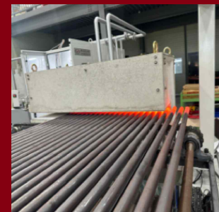
Partial Heater
